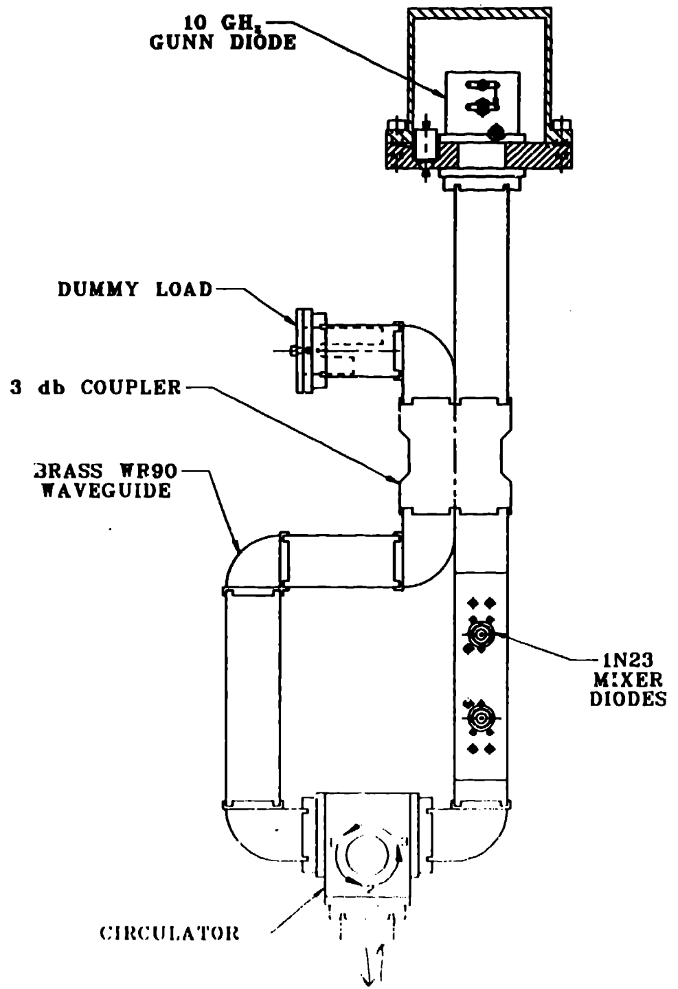
Fig 1. Microwave Mixer (Completed)
